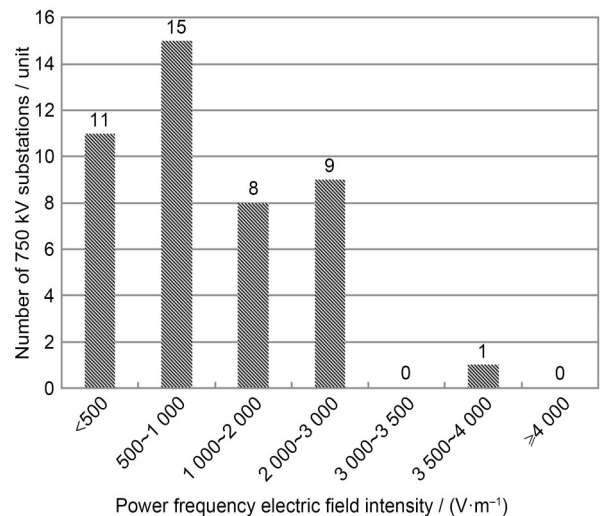
图3 750 kV 变电站监测断面工频电场强度最大值统计一览图 Fig.3 Statistical diagram of the max PFEF intensity at the monitoring section of 750 kV substation
